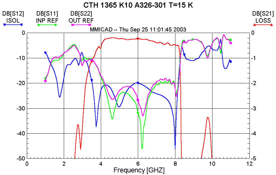
Figure 4: Isolator PAMTECH CTH 1365 K10 S/N 301.
