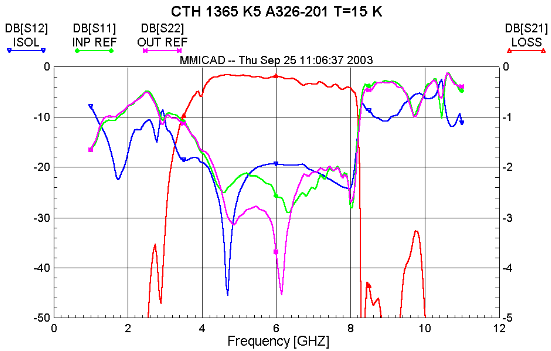
Figure 2: Isolator PAMTECH CTH 1365 K5 S/N 201.
