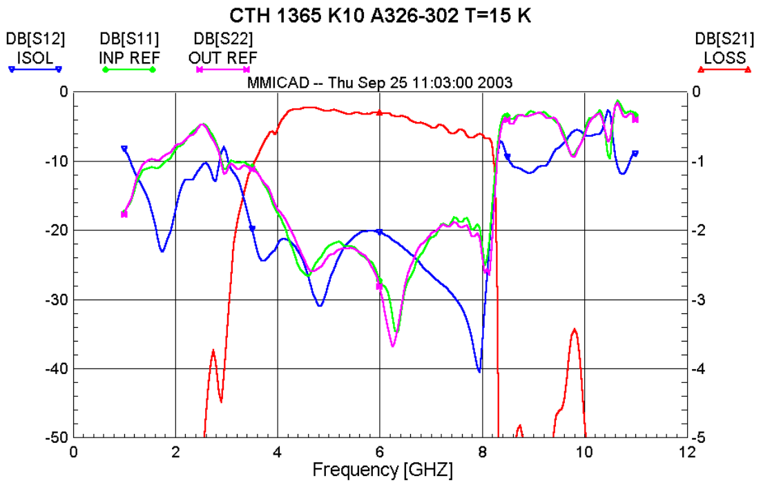
Figure 5: Isolator PAMTECH CTH 1365 K10 S/N 302.
