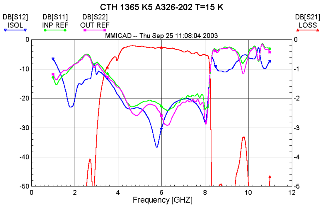
Figure 3: Isolator PAMTECH CTH 1365 K5 S/N 202.
